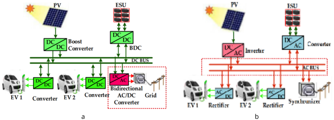
Figure 4. Renewable energy integrated Electric vehicle charging station (a) DC bus coupled, (b) AC bus coupled
