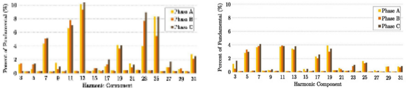
Figure 2. Input current harmonics (a) when input power is 11 kW, (b) when input power is 50
