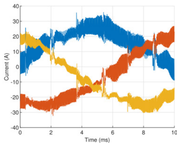
Figure 3. Supraharmonics in 3 phase input current of DC fast charger
