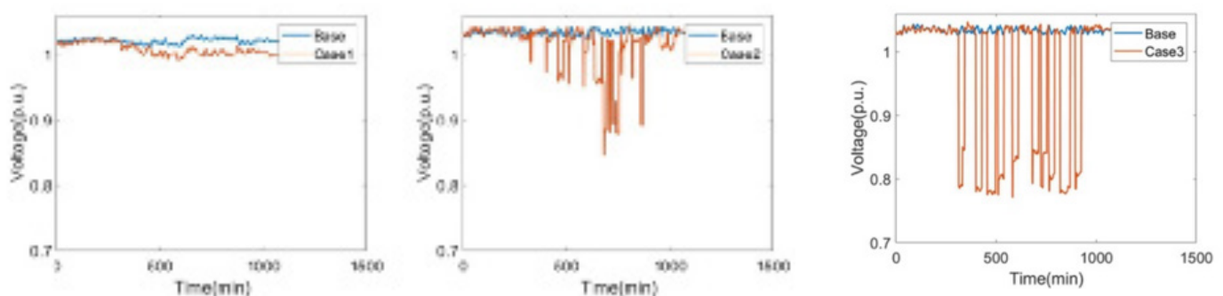
Figure 1. Voltage profile after charging station is connected
