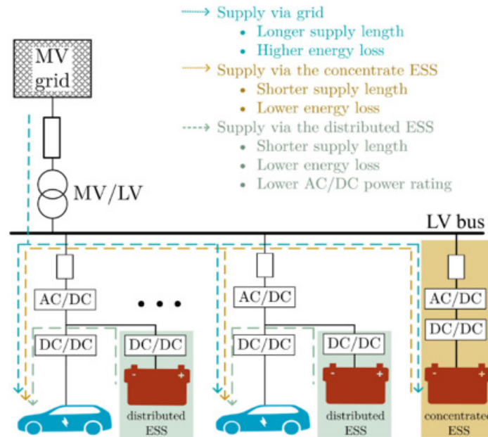
Figure 4. Energy storage integrated EV charging station
